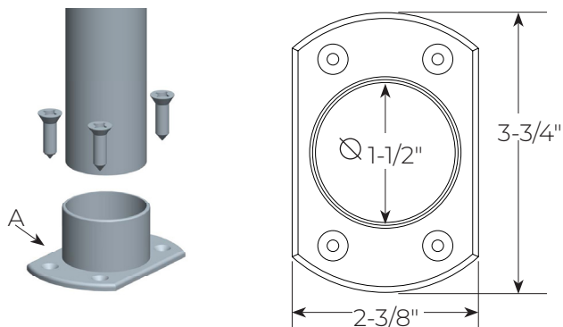
1-1/2" Narrow Flange
