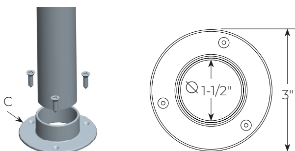
1-1/2" Round Flange
