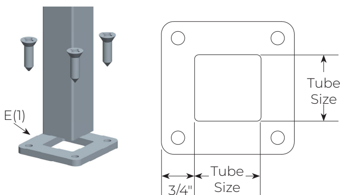
Square Flange
