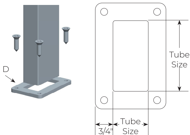
Rectangular Flange
